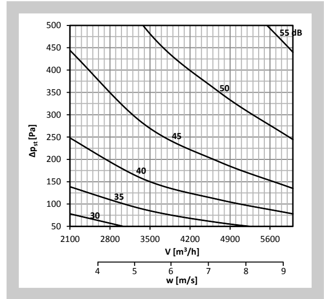
Diagram No. 68 Sound power level L_{WA} [dB(A)] radiated outside the pipeline 600x500, with insulation
