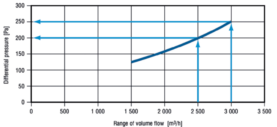
Standard HEPA-filter element 610/610/292 [mm], initial pressure at flow rate 3,000m 3 /h ≤ 250 Pa
