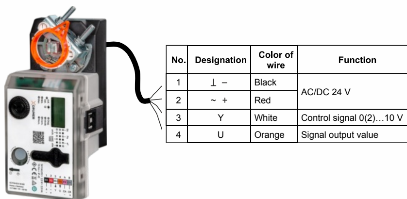
Fig. 19 Regulators 327VM-024-... -MB
