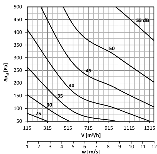
Diagram No. 24 Sound power level L_{WA} [dB(A)] radiated outside the pipeline DN250, without insulation
