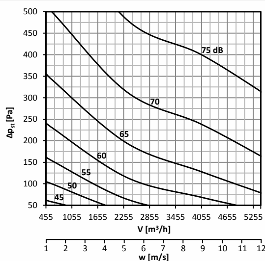
Diagram No. 15 Sound power level L_{WA} [dB(A)] inside the pipeline DN630
