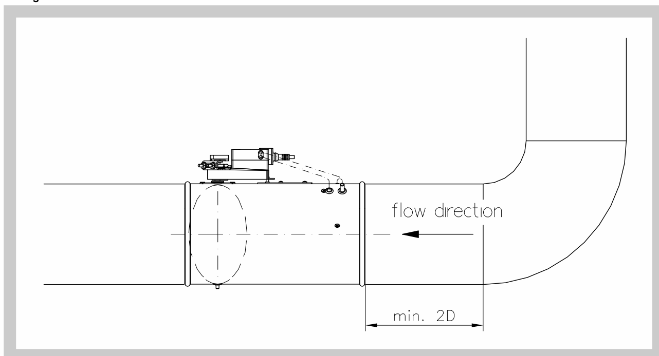
Fig. 34 Recommended distance from bend
