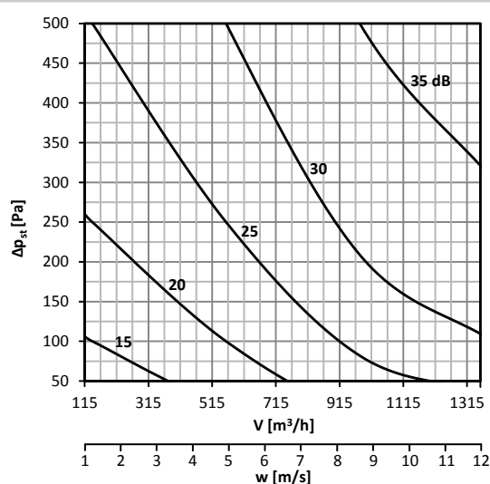
Diagram No. 39 Sound power level L_{WA} [dB(A)] radiated outside the pipeline DN250, with insulation
