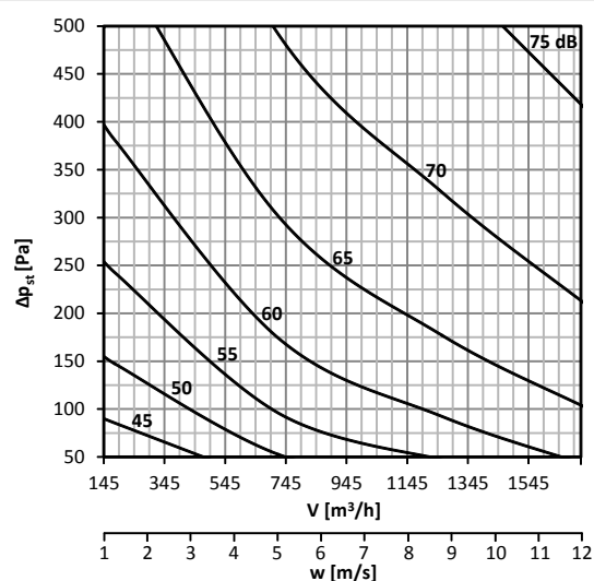
Diagram No. 10 Sound power level L_{WA} [dB(A)] inside the pipeline DN280
