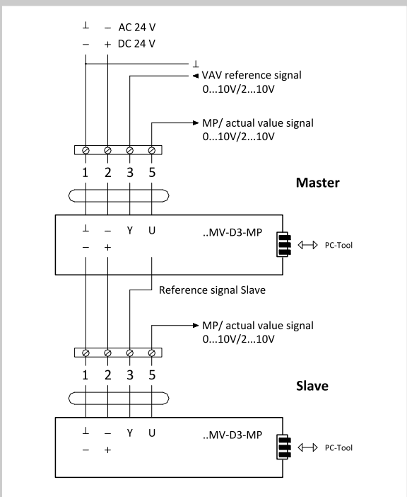
Fig. 8 Master-slave flow control with actuators LMV-D3-MP, NMV-D3-MP and SMV-D3-MP
