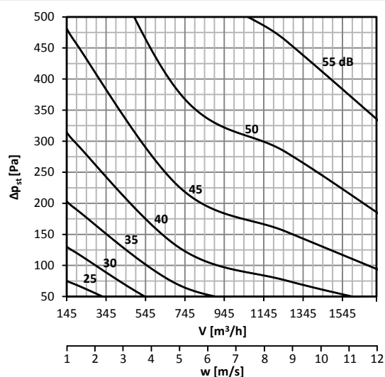
Diagram No. 25 Sound power level L_{WA} [dB(A)] radiated outside the pipeline DN280, without insulation
