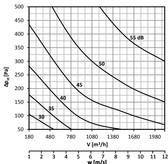
Diagram No. 26 Sound power level L_{WA} [dB(A)] radiated outside the pipeline DN315, without insulation
