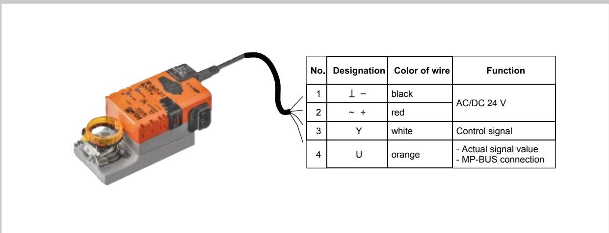
Fig. 6 Regulator LMV-D3-MP, NMV-D3-MP and SMV-D3-MP
