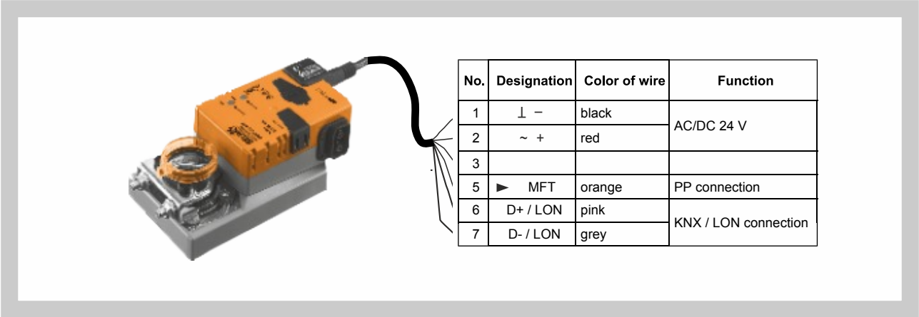
Fig. 11 Actuators LMV-D3-KNX, NMV-D3-KNX, LMV-D3-LON and NMV-D3-LON
