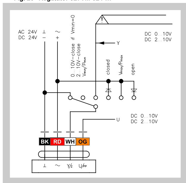
Fig. 20 Regulator 327VM-024-...
