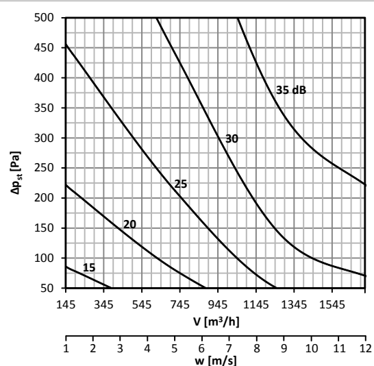
Diagram No. 40 Sound power level L_{WA} [dB(A)] radiated outside the pipeline DN280, with insulation
