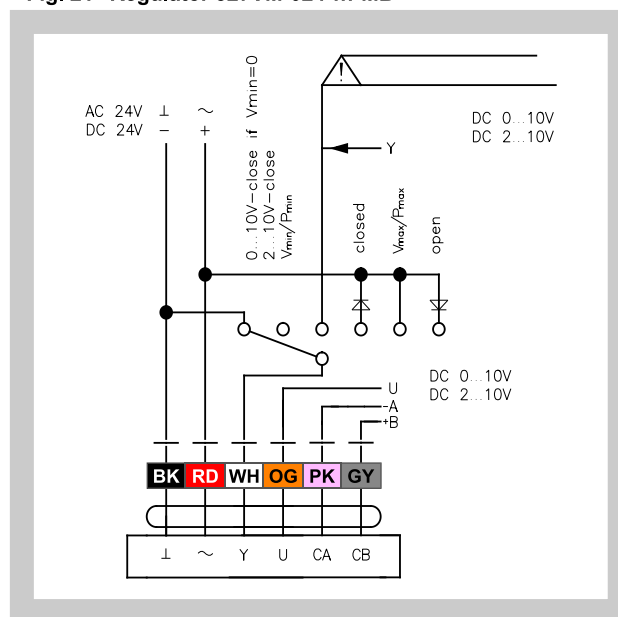
Fig. 21 Regulator 327VM-024-...-MB
