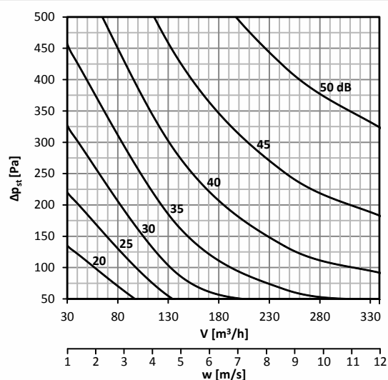
Diagram No. 19 Sound power level L_{WA} [dB(A)] radiated outside the pipeline DN140, without insulation
