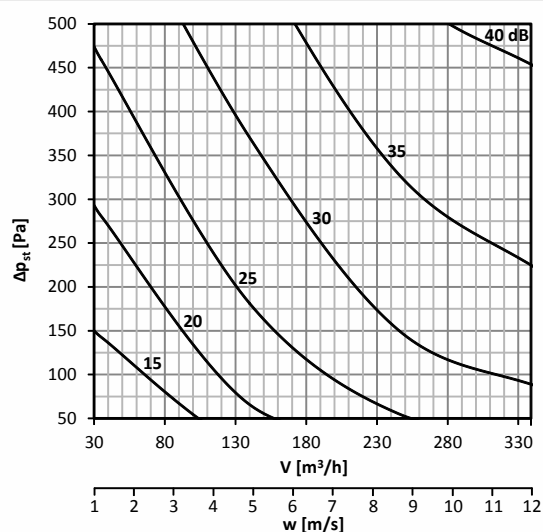
Diagram No. 34 Sound power level L_{WA} [dB(A)] radiated outside the pipeline DN140, with insulation
