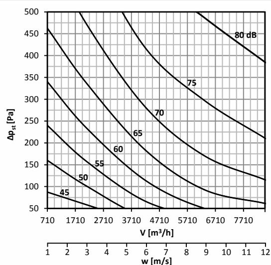
Diagram No. 14 Sound power level L_{WA} [dB(A)] inside the pipeline DN500
