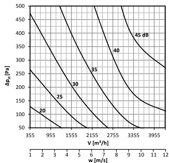
Diagram No. 42 Sound power level L_{WA} [dB(A)] radiated outside the pipeline DN355, with insulation
