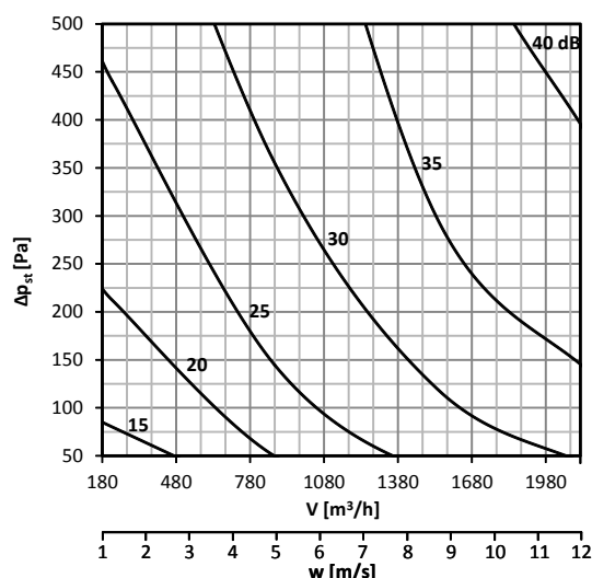
Diagram No. 41 Sound power level L_{WA} [dB(A)] radiated outside the pipeline DN315, with insulation
